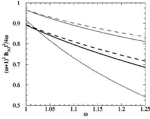
FIG. 1. The upper bound on (\omega+1)^2 |h_{A_1}(\omega)|^2 / (4\omega) . The thick solid (dashed) curve is the new (old) upper bound to \mathcal{O}(1/m_Q^2) including perturbative corrections. The thin solid (dashed) curve is the upper bound to \mathcal{O}(1/m_Q^2) without perturbative corrections. The dotted line is the lower bound to \mathcal{O}(1/m_Q) including perturbative corrections.
